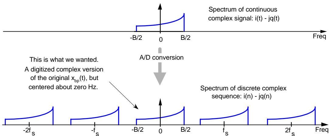
Figure 18. The continuous complex signal i(t) - jq(t) is digitized to obtain discrete i(n) - jq(n) .
