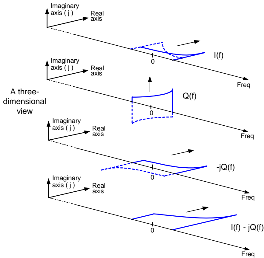
Figure 17. 3-D view of combining the I(f) and Q(f) spectra to obtain the I(f) - jQ(f) spectra.
